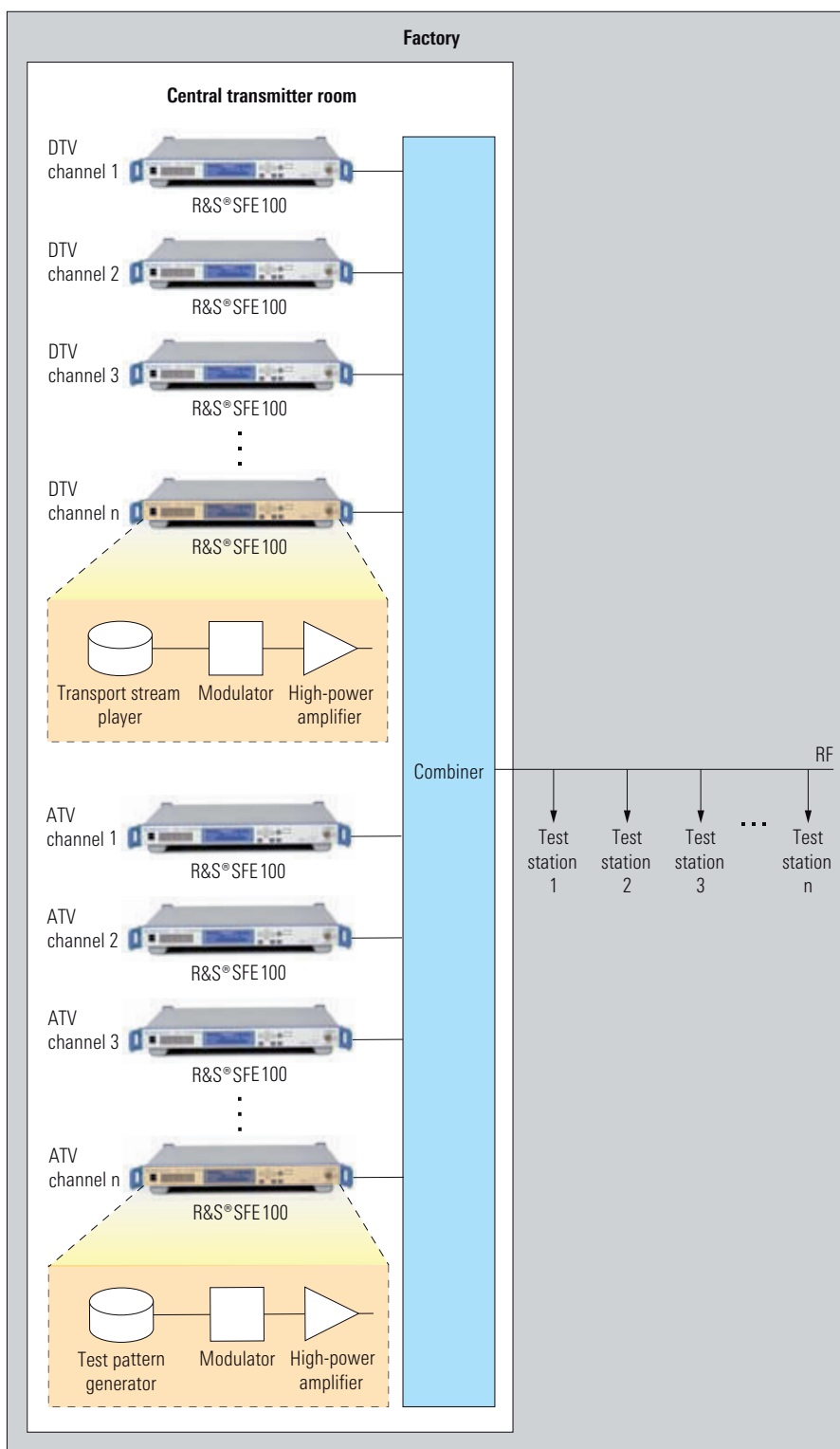
Schematic picture of a central transmitter room
